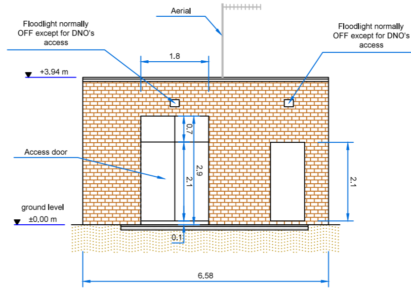
front elevation
