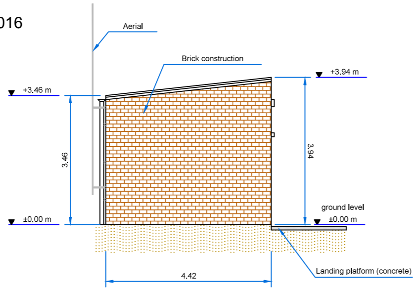
side 1 elevation
