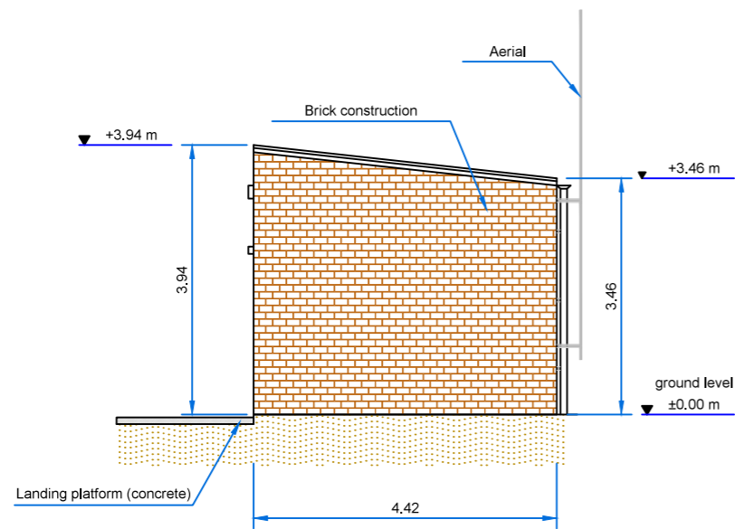
side 2 elevation
